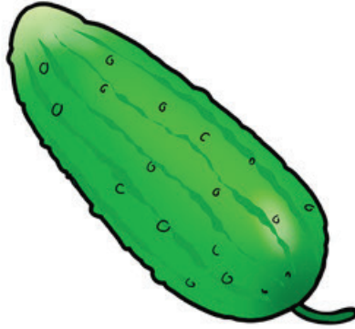
Cucumber
