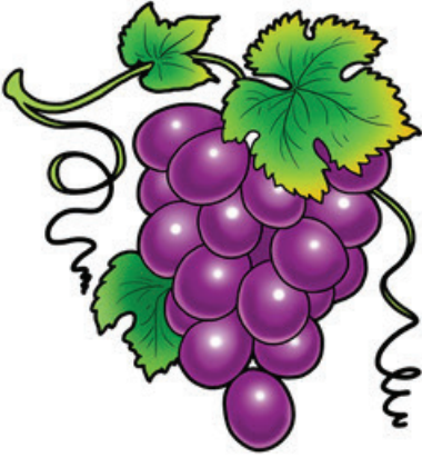
Grape
