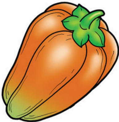
Bell pepper
